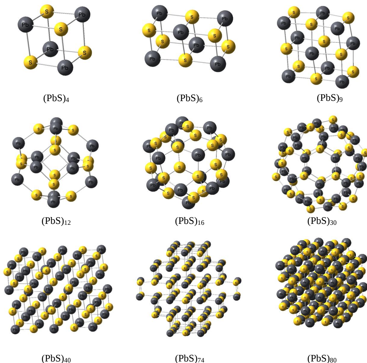
Supplementary 1: Optimized geometries of PbS i.e., (PbS) 4 , (PbS) 6 , (PbS) 9 , (PbS) 12 , (PbS) 16 , (PbS) 30 , (PbS) 40 , (PbS) 74 and (PbS) 80 .
