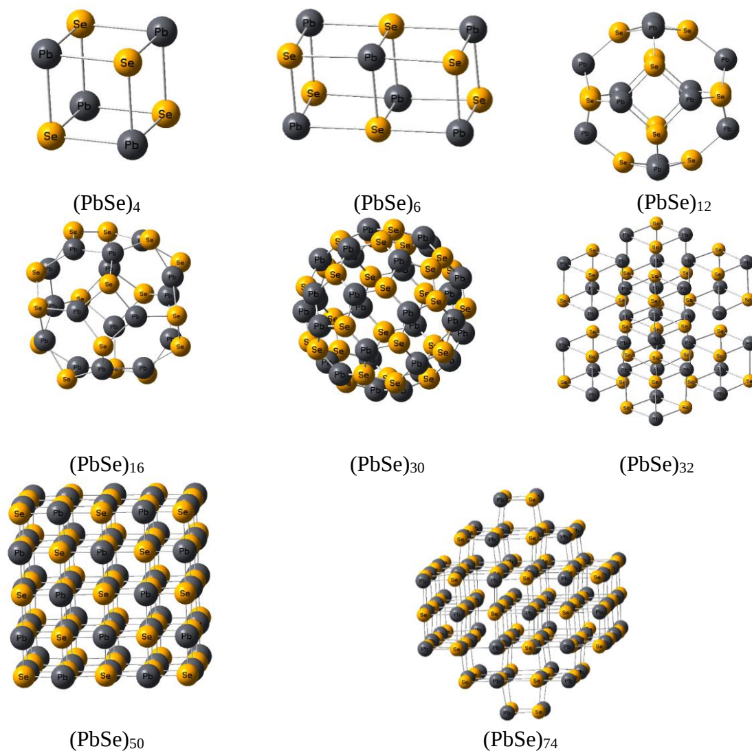
Supplementary 2: Optimized geometries of PbSe i.e., (\text{PbSe})_4 , (\text{PbSe})_6 , (\text{PbSe})_{12} , (\text{PbSe})_{16} , (\text{PbSe})_{30} , (\text{PbSe})_{32} , (\text{PbSe})_{50} and (\text{PbSe})_{74} .
