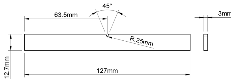
Figure 2: Specimen size for Charpy impact test
