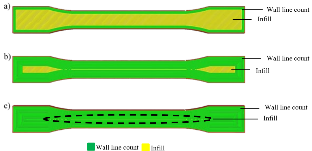
Figure 3: The illustration showing the wall line count arrangement for tensile test specimen with wall line count of (a) 6 layers, (b) 18 layers and (c) 30 layers
